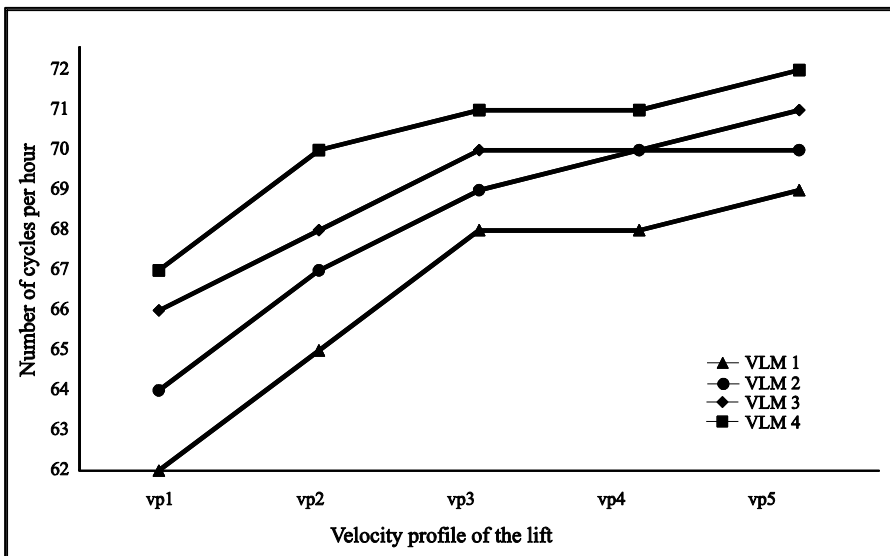
Figure 6: VLM performance in number of trays per hour when t_{pick} = 30 sec.
