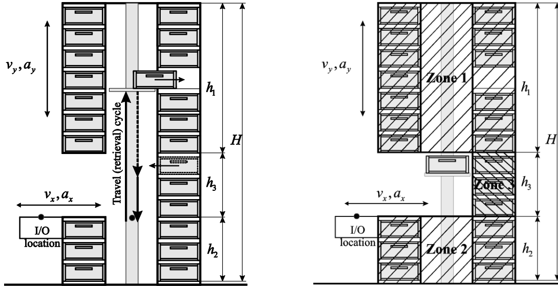
Figure 2: Definition of the travel (retrieval) cycle and zoning of the VLM.
