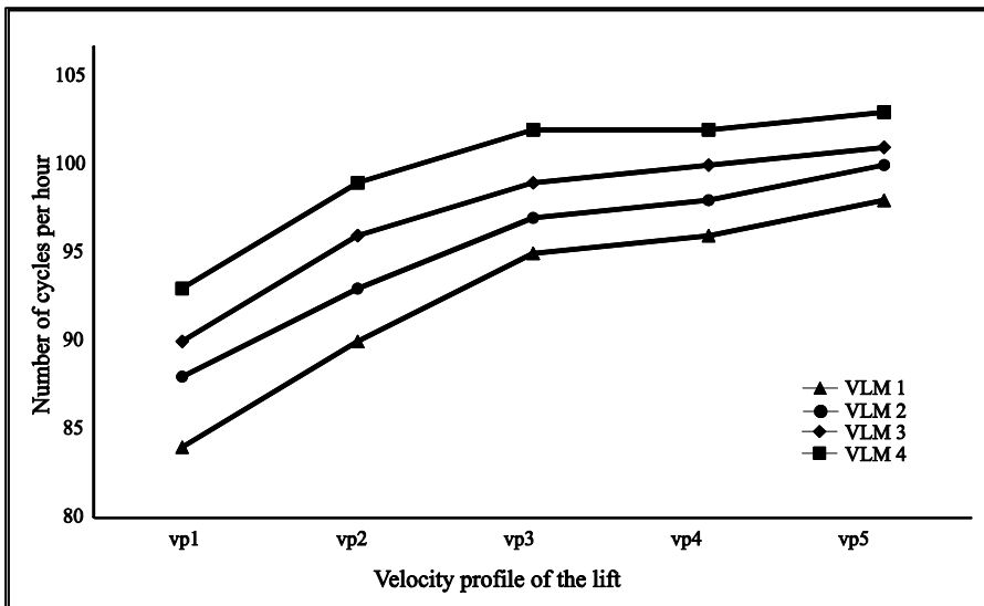
Figure 5: VLM performance in number of trays per hour when t_{pick} = 15 sec.
