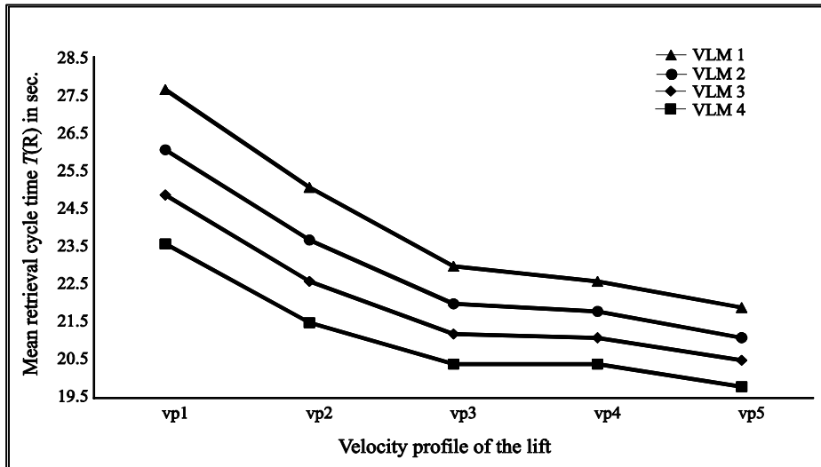
Figure 3: VLM cycle (retrieval) time analysis.
