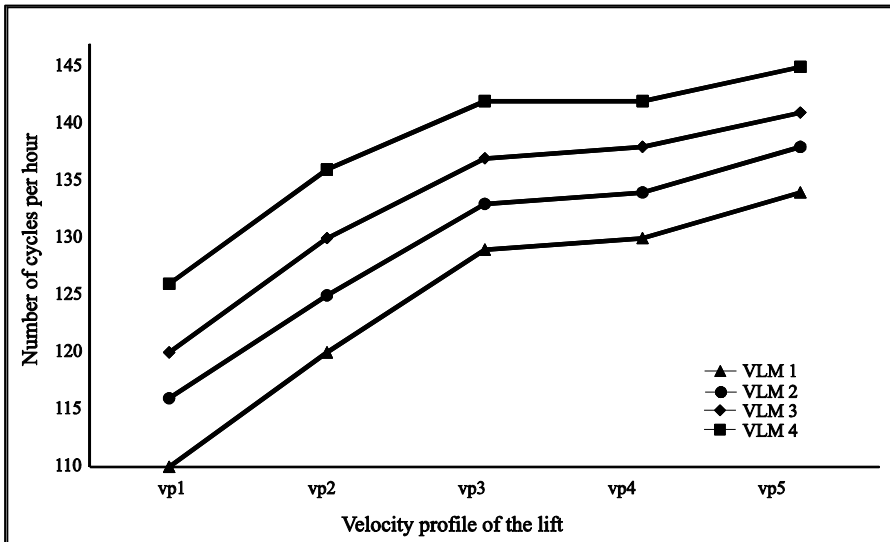
Figure 4: VLM performance in number of trays per hour when t_{pick} = 5 sec.
