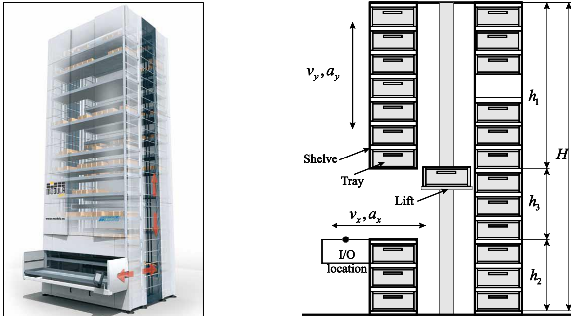
Figure 1: Vertical lift module of the material handling provider MODULA ( http://www.modula.eu/ ).
